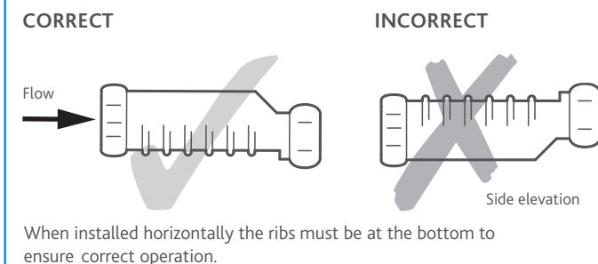
6 MVHR-DRAIN Installation
