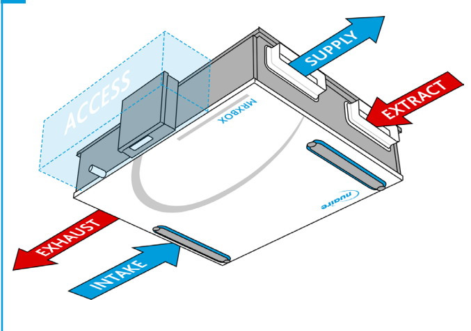
2 Opposite Handed Unit Duct Configuration
