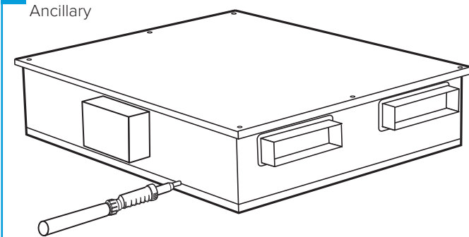
6 MVHR-DRAIN Installation
