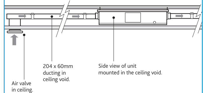
4 Side View Of Standard Unit Typical Ceiling Void Installation Using 204 x 60 mm Rectangular Ducting & Air Valves
