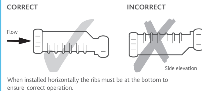
6 MVHR-DRAIN Installation
