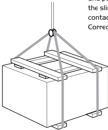
Figure 1. Lifting unit with slings via spreaders.
