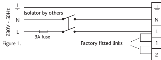
Figure 1. Basic wiring. Both supply and extract will run at constant speed. The fan duty is controlled via the 'Boost' setting.
