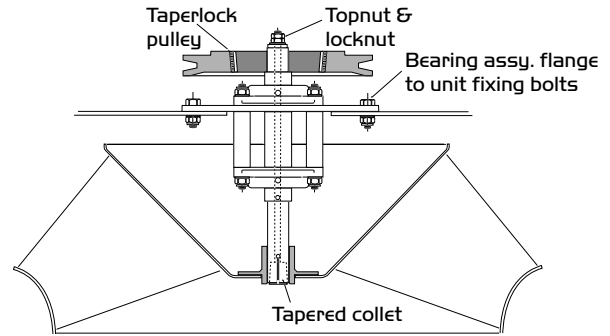
Figure 11. The impeller, bearing and pulley
