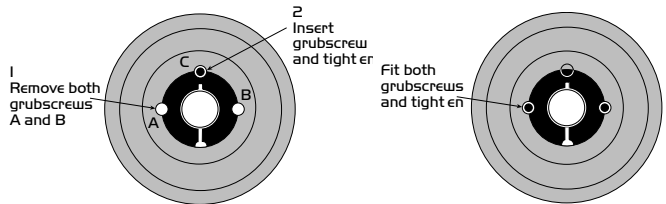
Figure 12. Removing and fitting the Taperlock pulley
