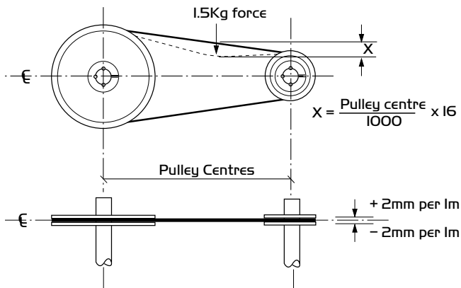
Figure 10. Belt/Pulley adjustment
