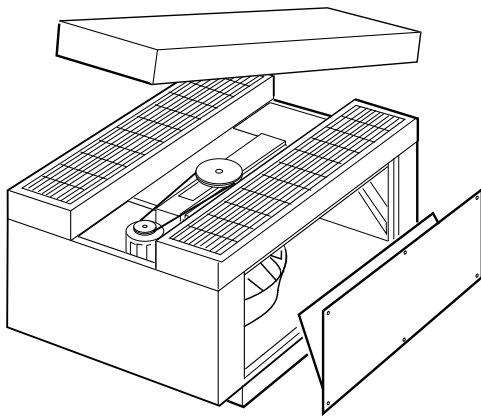
Figure 9. Access for maintenance
