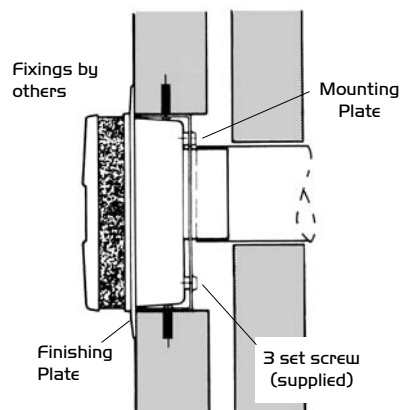
Figure 5. Semi-recessed mounted, wall.
