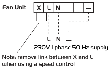
Figure 5. Single phase electronic speed control.
