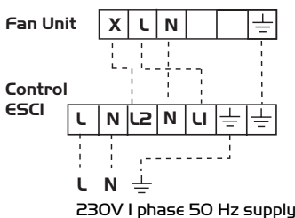
Figure 5. Single phase electronic speed control.
