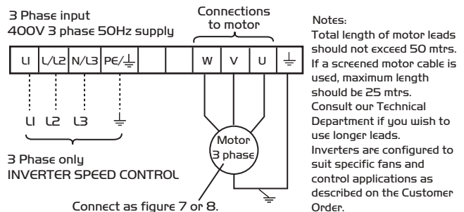
Figure 11. 3 phase units with matched frequency inverter.
