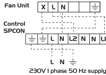
Figure 6. Single phase transformer speed control.
