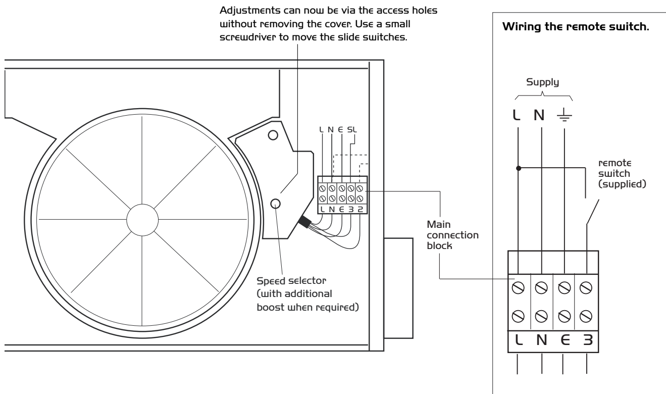
Figure 1. Customer installation wiring.
